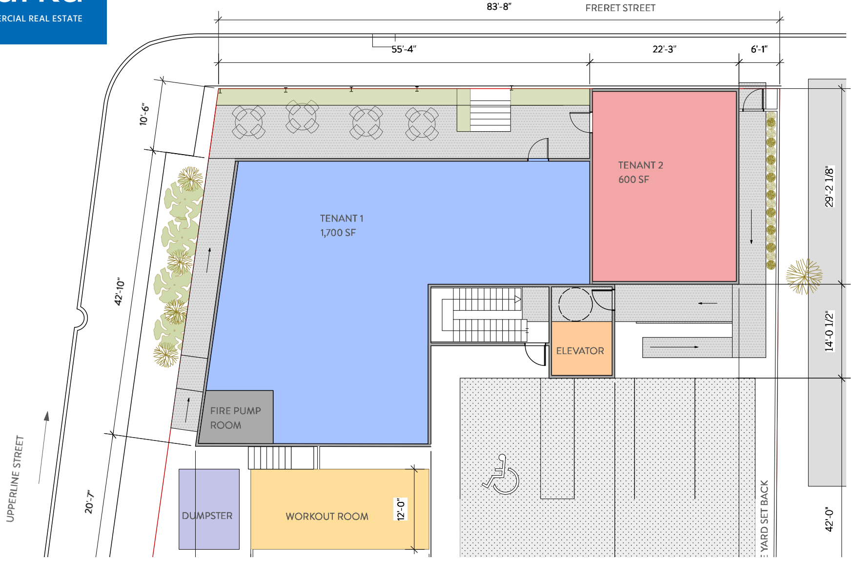
FLOOR PLAN
